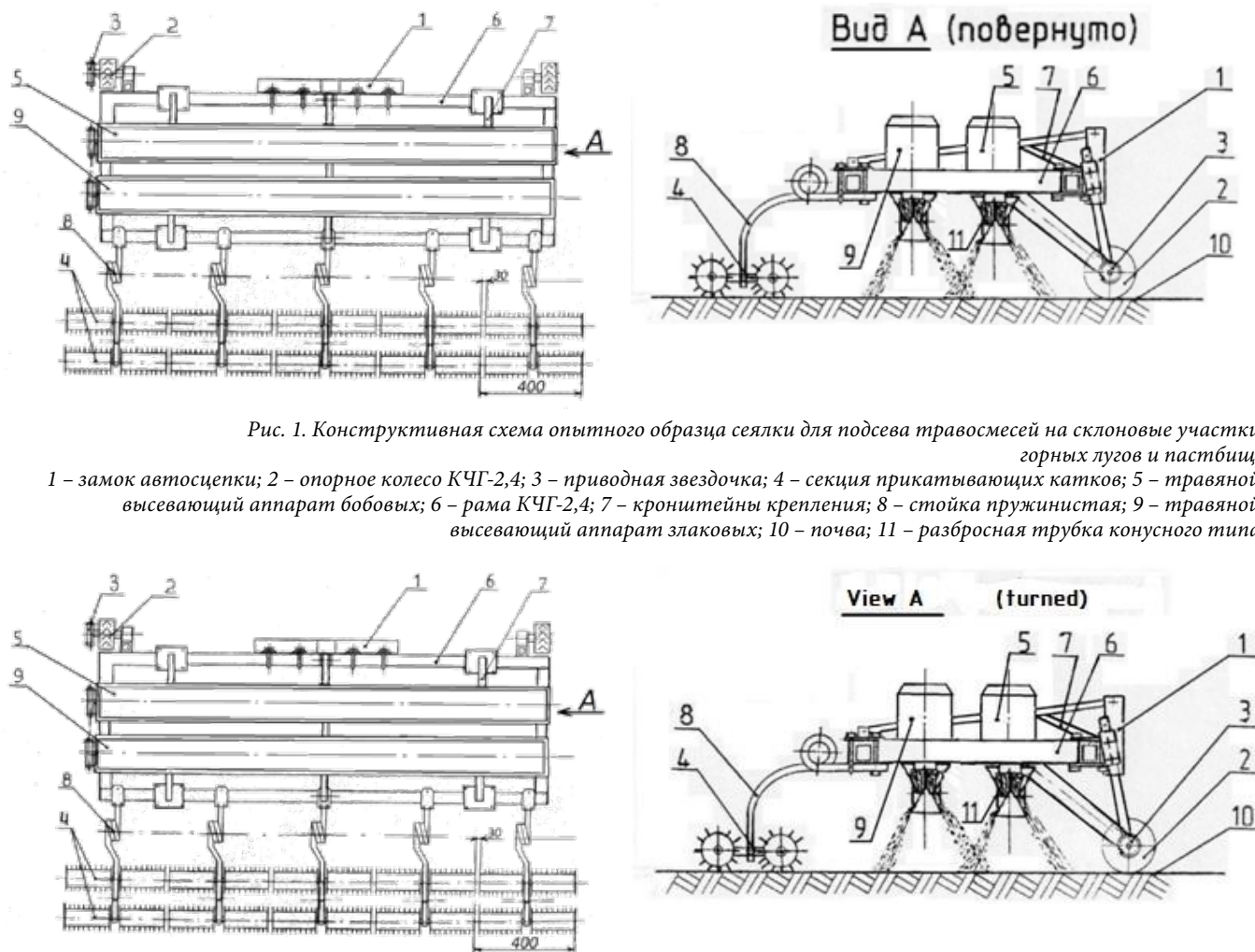
Fig. 1. Constructive diagram of the experimental sample of a seeder for sowing grass mixtures on slopes of mountain meadows and pastures: 1 – automatic coupler; 2 – support wheel KCHG-2,4; 3 – a drive asterisk; 4 – section of compacting rollers; 5 – herbal sowing machine of legumes; 6 – frame KCHG-2,4; 7 – mounting brackets; 8 – the rack is spring-loaded; 9 – herbal sowing device cereals; 10 – soil; 11 – spreading tube of conical type
